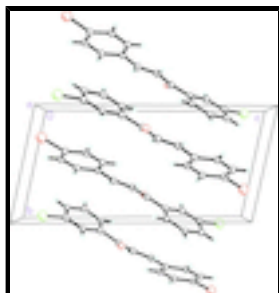
Fig. 2. Packing diagram of the title compound, (I), viewed down the a axis.
